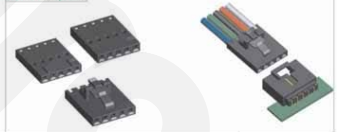
3750X-XX No. Of Contacts (2 To 12 Ways) A: Flat Type Housing C: W/Guide Housing G: W/Lock Housing
