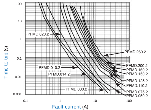
Typical Time to Trip at 23 °C
