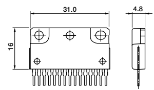
SLA15pin
