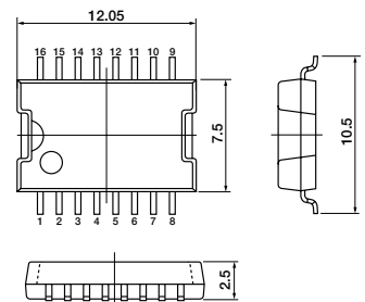
SPF16pin
