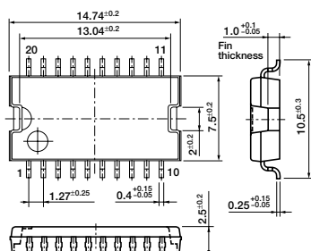
SPF20pin
