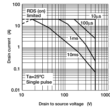
Safe operating area (Power MOS FET)
