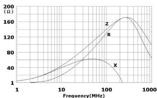
FBU453215T-151Y-S
