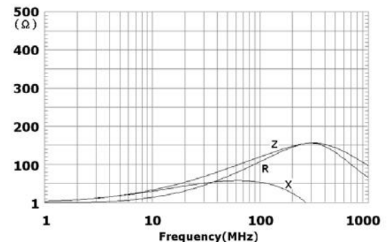
FBU201209T-121Y-S
