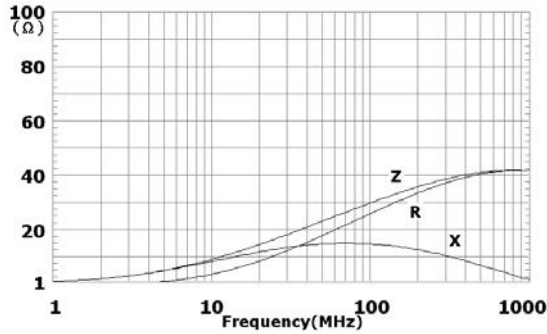
FBU321611T-800Y-S
