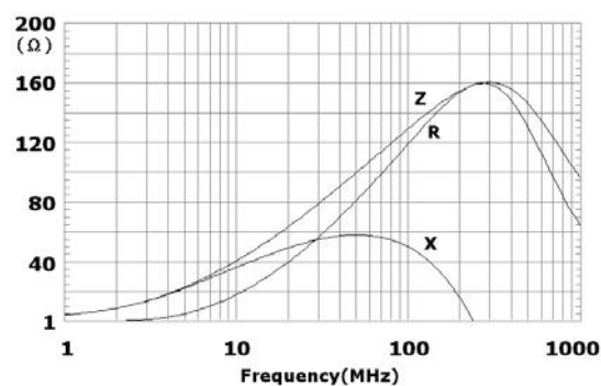
FBU453215T-121Y-S
