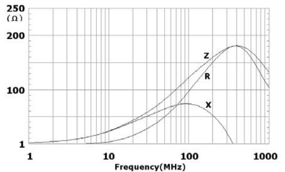
FBU322513T-600Y-S
