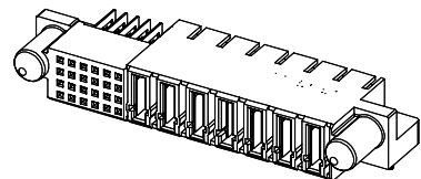
87700 Right Angle, Through Hole Receptacle
