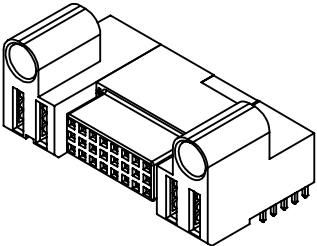
46436 Right Angle, Through Hole Receptacle
