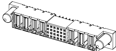
87734 Vertical, Through Hole Receptacle
