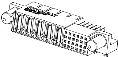
87668 Right Angle, Through Hole Receptacle
