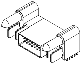
46437 Right Angle, Through Hole Header
