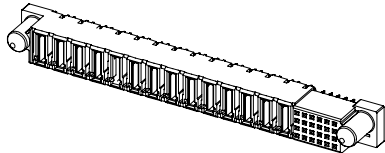
87710 Vertical, Press-Fit Receptacle
