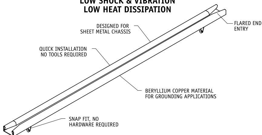
Series 38 SNAP-TAINER
