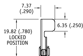
FINGER TAB OPTION NOT TO SCALE - LEFT HAND SHOWN
