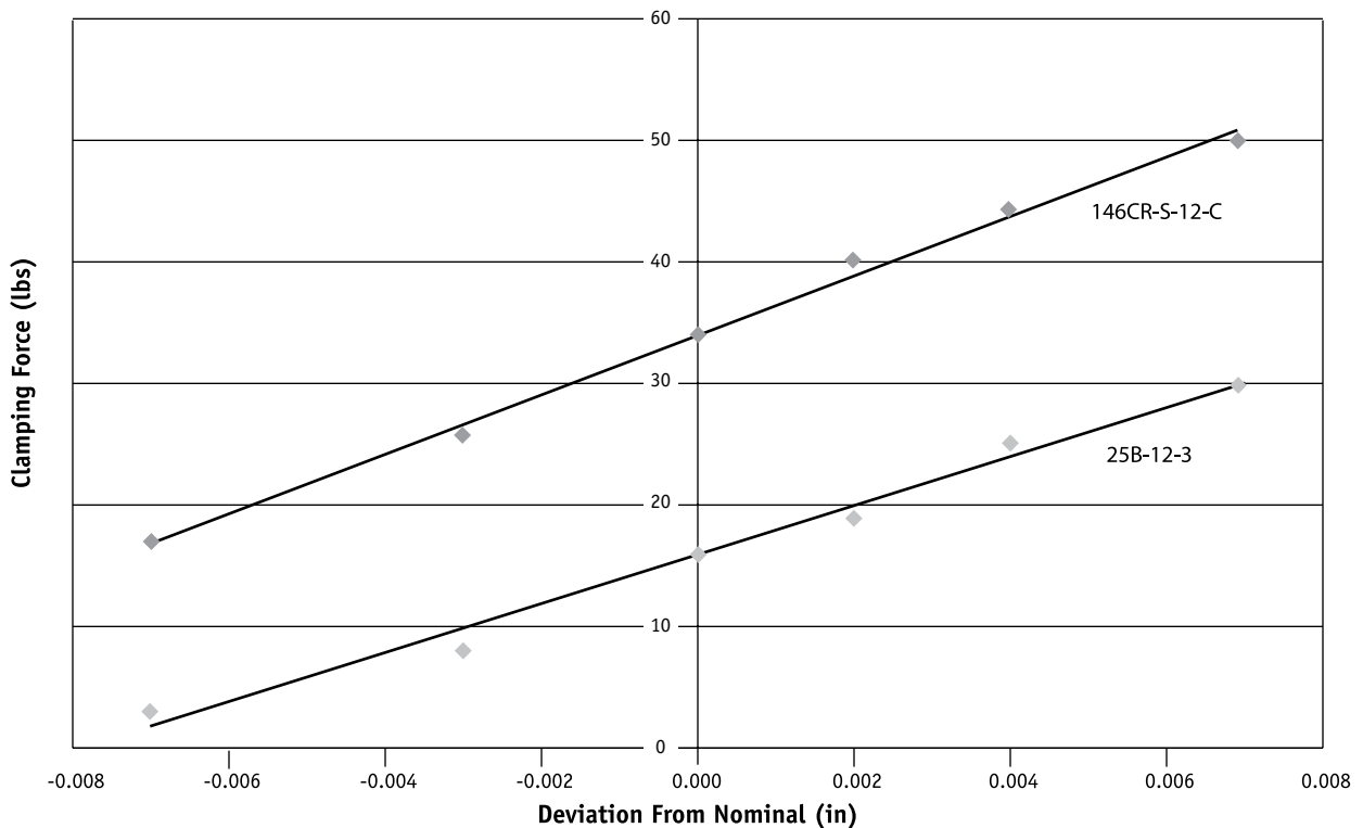
Figure 3. Effect of Board Thickness Tolerance on Clamping Force for Lever-actuated Card Guides
