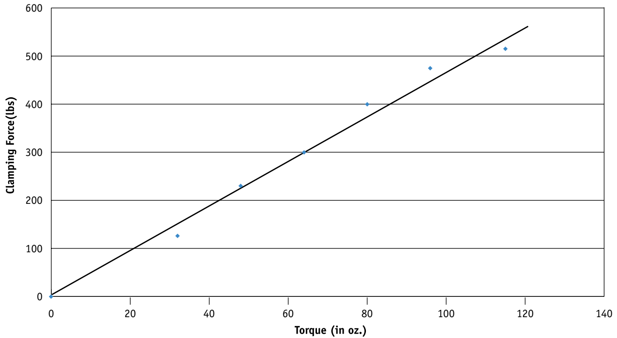
Figure 2. Clamping Force vs. Applied Torque 40-5-12-LF
