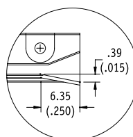
FLARED ENTRY OPTION DETAIL
