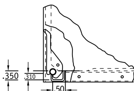
CARD CAGE FRONT CHANNEL DETAIL FOR SERIES 73 AND 87
