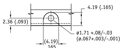
MOUNTING HOLE DETAIL NOT TO SCALE
