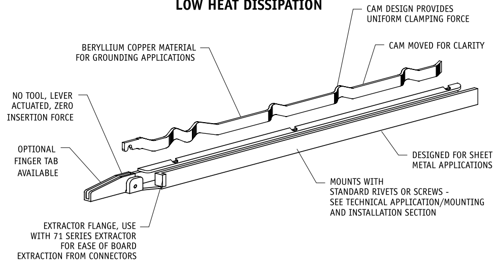
Series 24 LOK-TAINER
