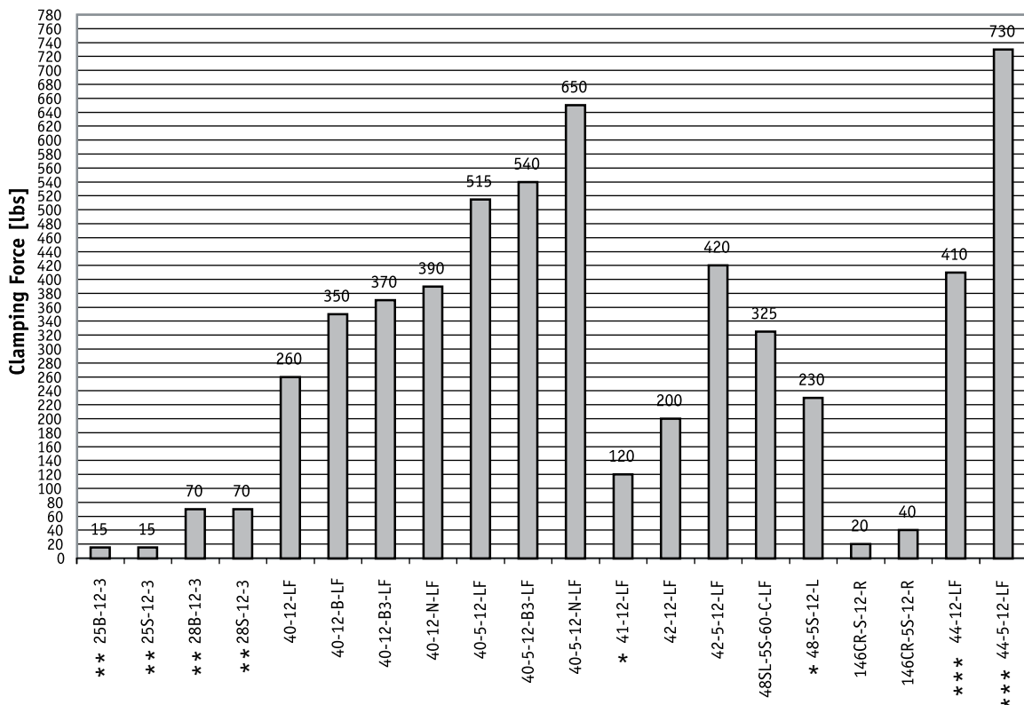
Figure 1. Clamping Force
