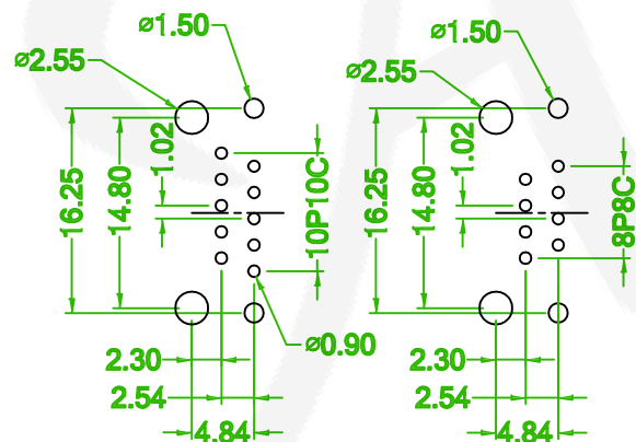
Recommended PCB Layout (PCB TOLERANCE \pm 0.05 )
