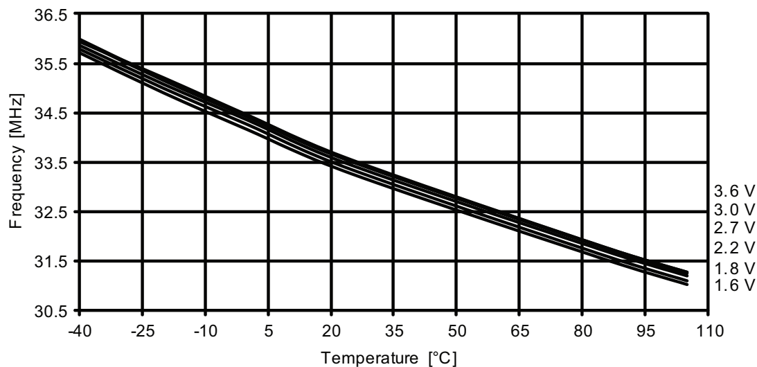
Figure 37-240. 32MHz internal oscillator frequency vs. temperature. DFLL disabled.
