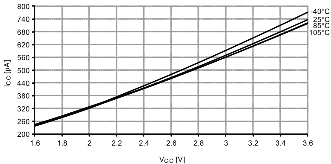
Figure 37-170. Active mode supply current vs. V_{CC} .
