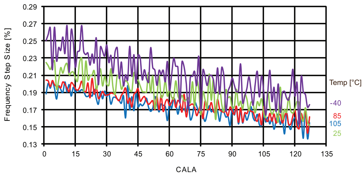
Figure 37-156. 2MHz internal oscillator CALA calibration step size.
