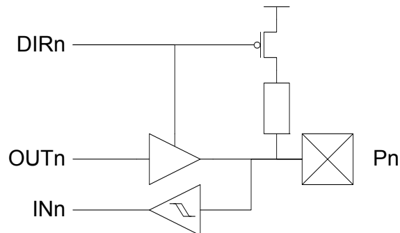
Figure 15-3. I/O configuration - Totem-pole with pull-up (on input).
