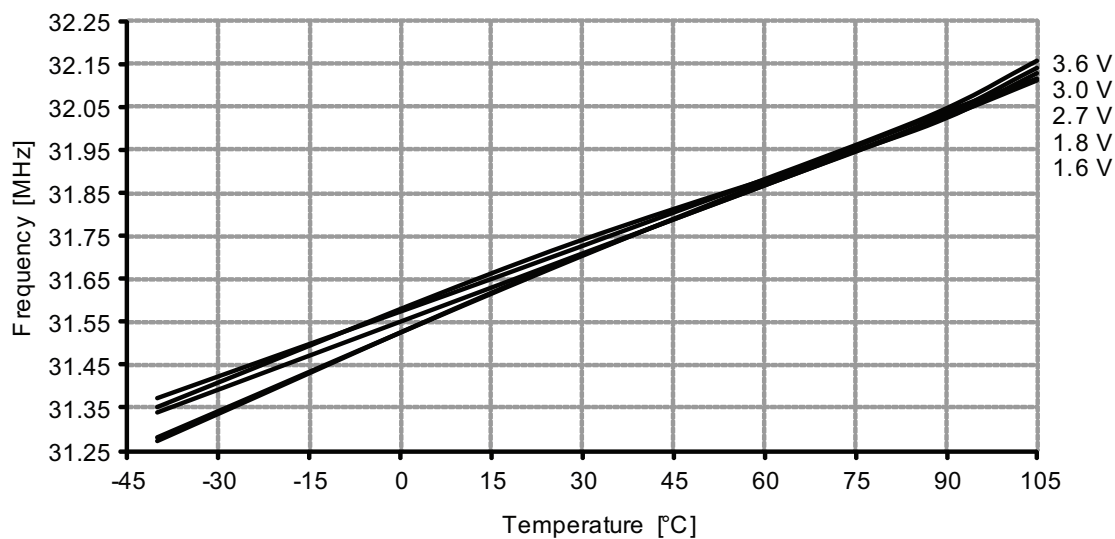
Figure 37-75. 32MHz internal oscillator frequency vs. temperature. DPLL enabled, from the 32.768kHz internal oscillator.
