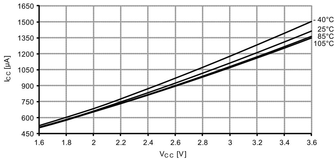
Figure 37-255. Active mode supply current vs. V_{CC} .
