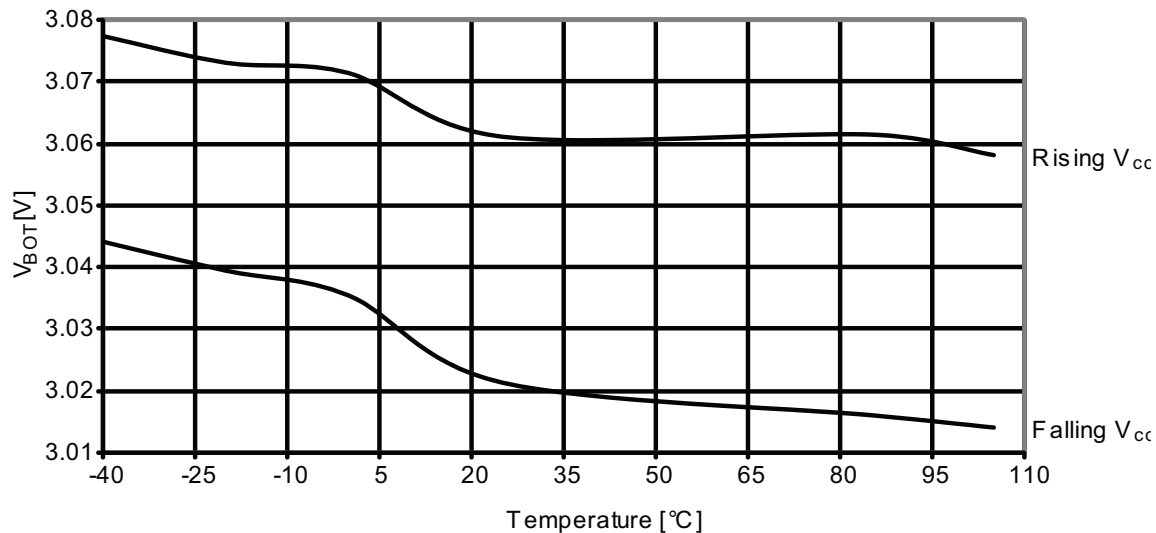
Figure 37-226. BOD thresholds vs. temperature.
