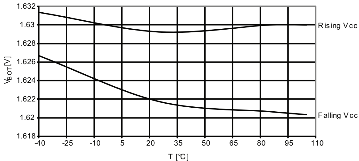
Figure 37-225. BOD thresholds vs. temperature.
