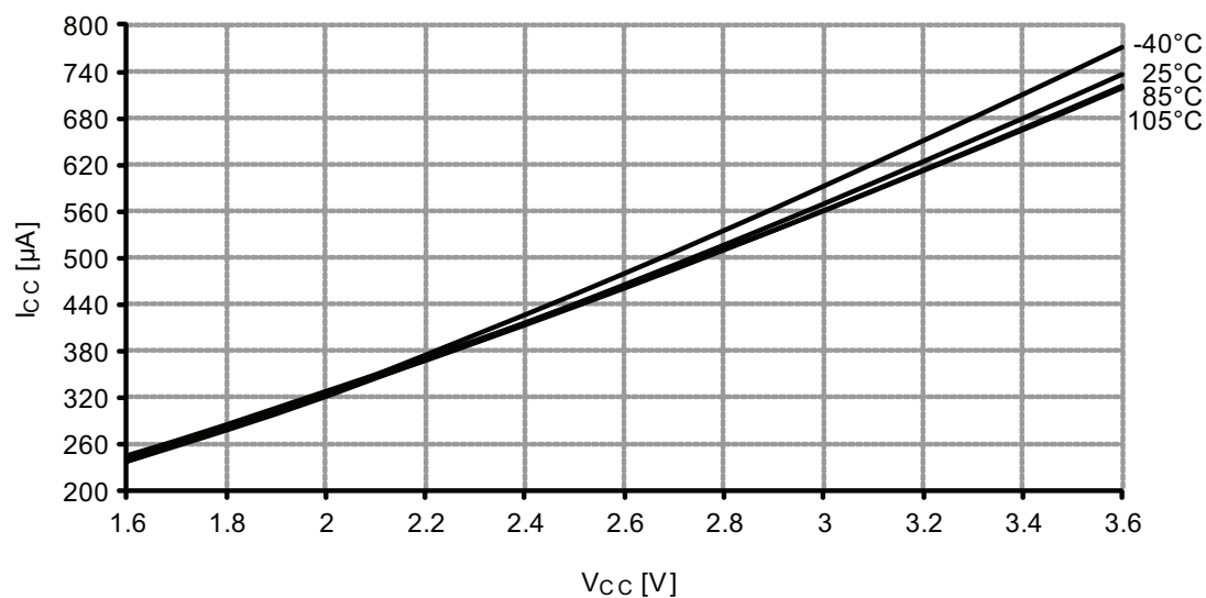
Figure 37-253. Active mode supply current vs. V_{CC} .
