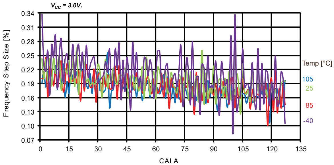
Figure 37-159. 32MHz internal oscillator CALA calibration step size.
