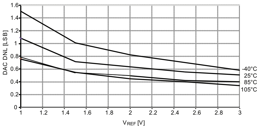
Figure 37-298. DNL error vs. V_{REF} . T = 25^{\circ}\text{C} , V_{CC} = 3.6\text{V} .
