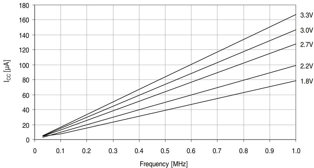
Figure 37-257. Idle mode supply current vs. frequency.
