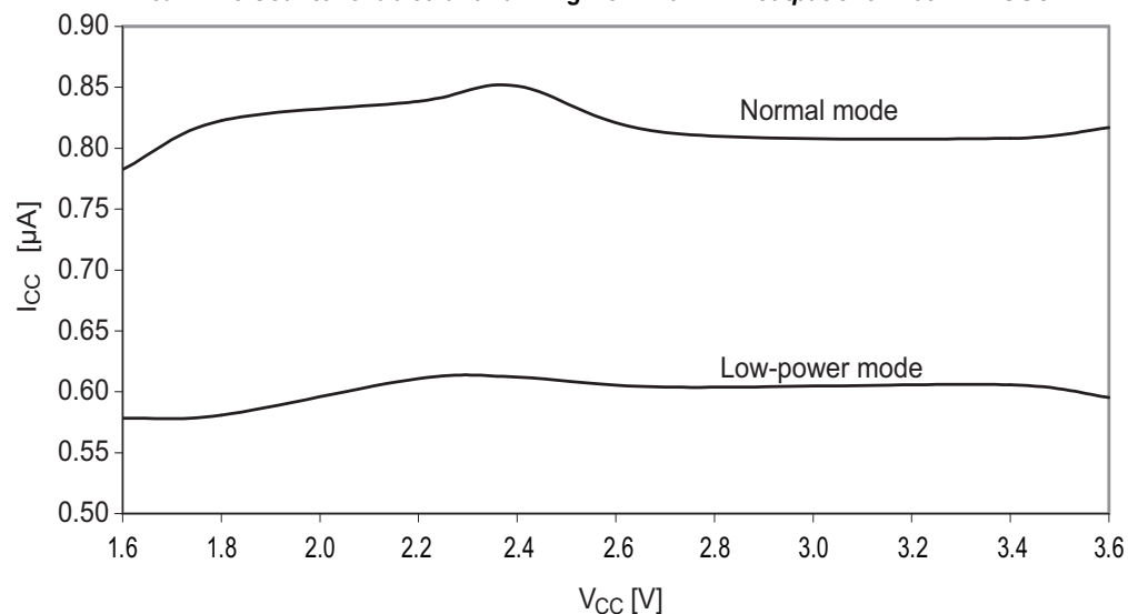
Figure 37-100. Power-save mode supply current vs. V_{CC} .
