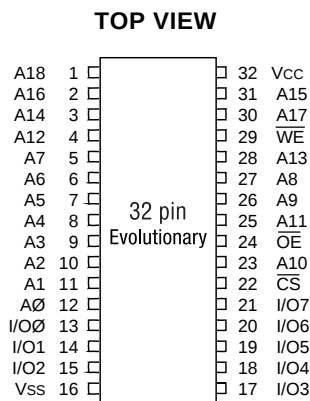
FIG. 1 PIN CONFIGURATION
