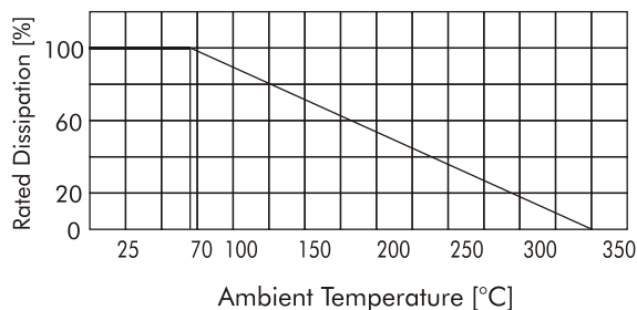
DERATING CURVE
