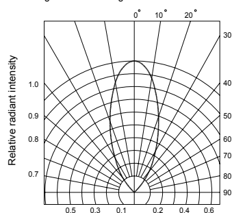
Fig.6 Radiation diagram
