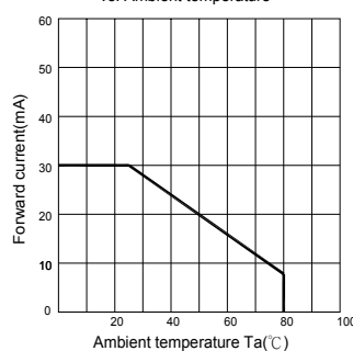
Fig.2 Forward current derating curve vs. Ambient temperature
