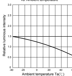
Fig.4 Relative luminous intensity vs. Ambient temperature
