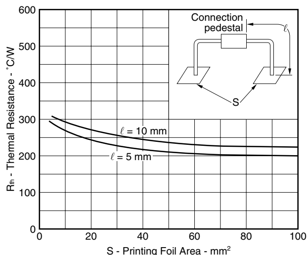
Figure 2. R_{th} vs. S Example of Characteristics
