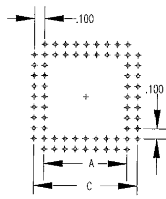
PCB LAYOUT
