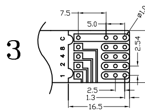
Extended P.C.B Pitch=2.54
