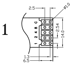
General P.C.B Pitch=2.54
