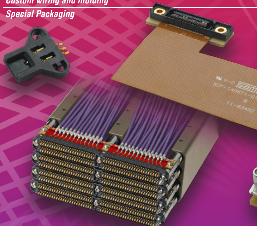
Combination coaxial grounds and open pin field array
