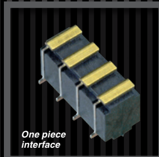
Special bends and selective gold plating
