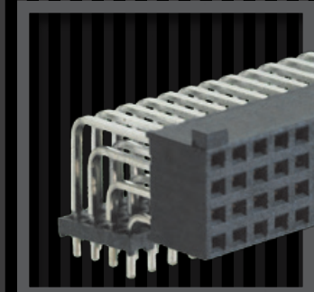
Special bends and selective gold plating
