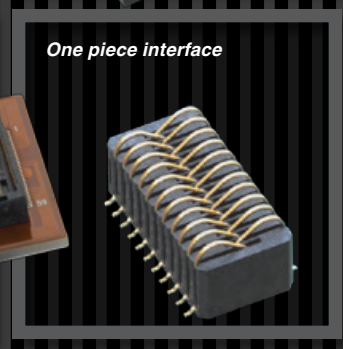
Custom bent pins and plating
