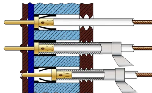
TYPICAL REAR RELEASE CONTACT
