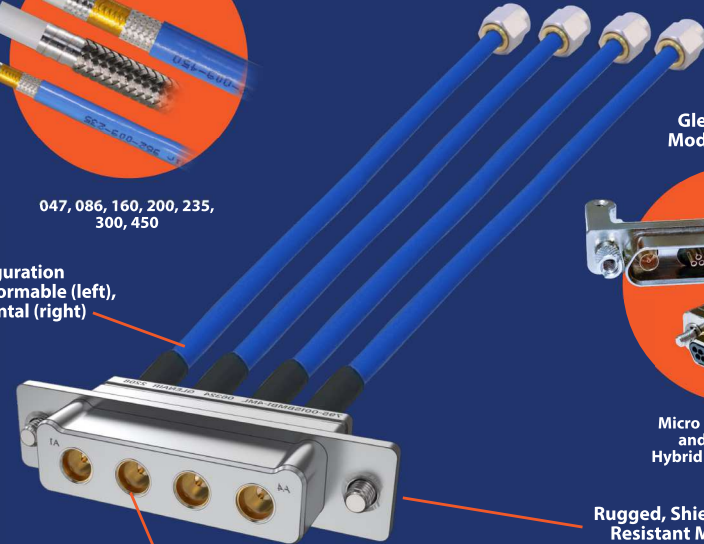
Single-Channel RF Connectors for Multi-Port Shell Configurations sizes #8, #12, #16
