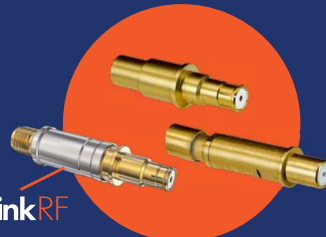
G-LinkRF: 26.5 GHz RF BMB-to-SMA contact adapters
