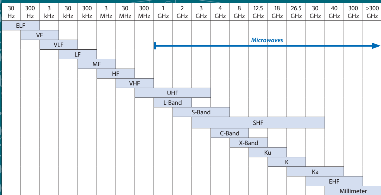
Relative positions of the most common frequency bands (not to scale).
