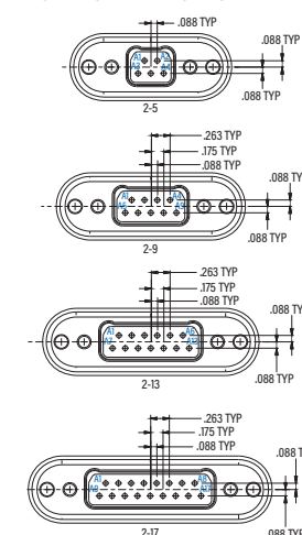
SINGLE ROW ARRANGEMENTS RECEPTACLE MATING FACE VIEW
