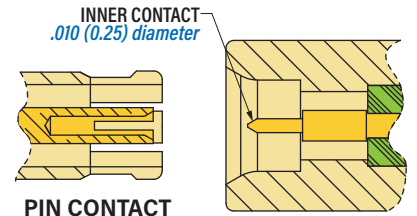
SOCKET CONTACT
