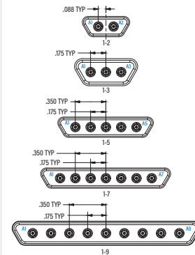
SINGLE ROW ARRANGEMENTS RECEPTACLE MATING FACE VIEW
