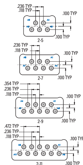
TWO ROW ARRANGEMENTS PLUG MATING FACE VIEW
