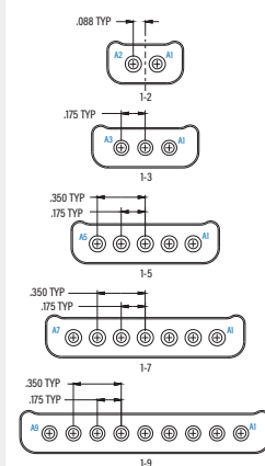
SINGLE ROW ARRANGEMENTS RECEPTACLE MATING FACE VIEW
