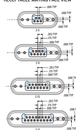
TWO ROW ARRANGEMENTS RECEPTACLE MATING FACE VIEW
