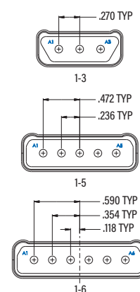
SINGLE ROW ARRANGEMENTS RECEPTACLE MATING FACE VIEW
