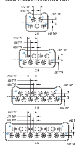
TWO ROW ARRANGEMENTS RECEPTACLE MATING FACE VIEW
