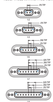
SINGLE ROW ARRANGEMENTS RECEPTACLE MATING FACE VIEW
