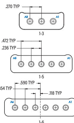
SINGLE ROW ARRANGEMENTS PLUG MATING FACE VIEW
