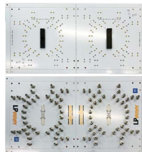
LP Array™ Low Profile Arrays (LPAM/LPAF)
