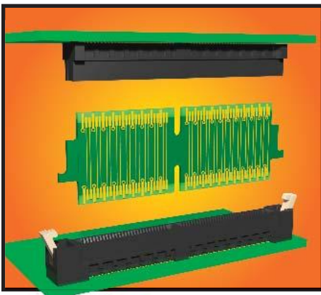
Board to connector lock (-BL option)
