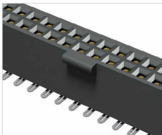
Locking for increased unmating force (SFML/TFML)
